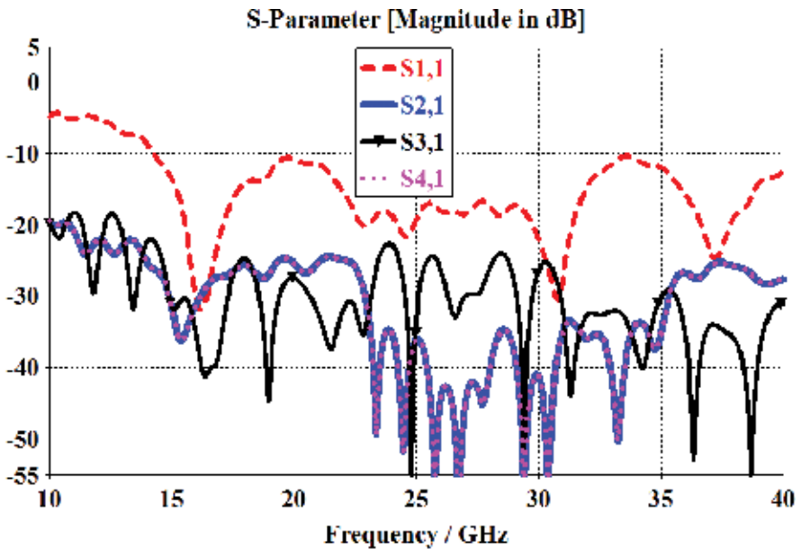
Figure 12. S-parameters of four-element beam-switched antenna system [38].
