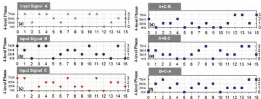
Figure 25. Measured symbol sequence for (a)–(c) three-input optical quaternary signal and their (c)–(e) addition/subtraction.
